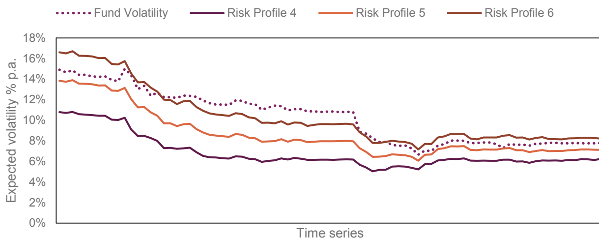
Figure 4: Observed volatility relative to Dynamic Planner over rolling one-year periods
